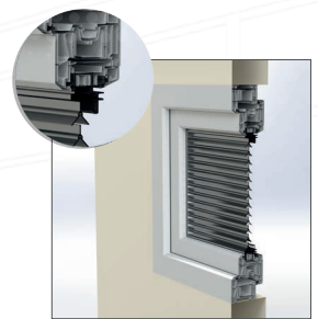
Glazed-in louvre
