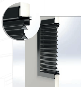
Flanged louvre
