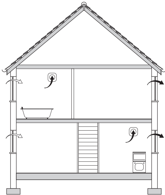
System 1 background ventilators and intermittent extract fans
