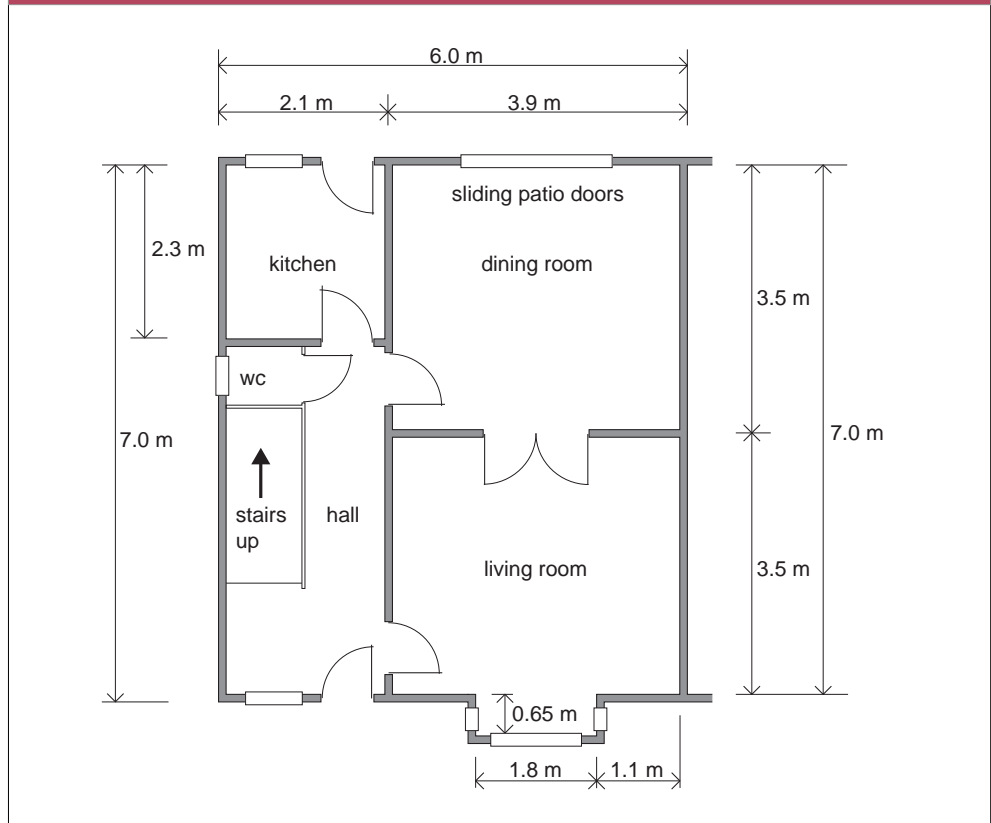
Diagram C2 Semi-detached house ground floor plan
