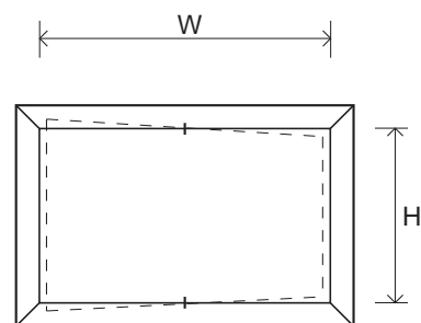
(b) Centre pivot (about vertical axis)
