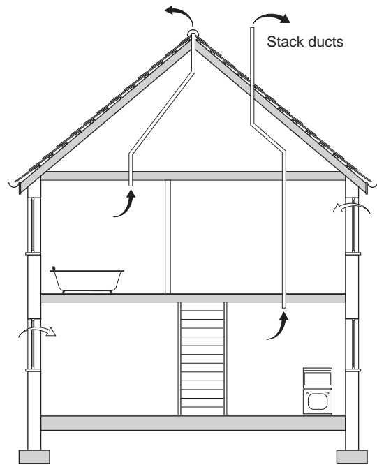
System 2 passive stack ventilation
