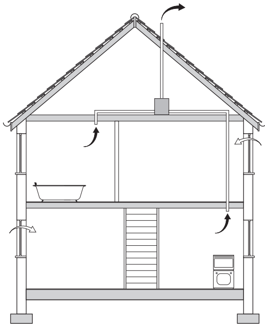
System 3 continuous mechanical extract
