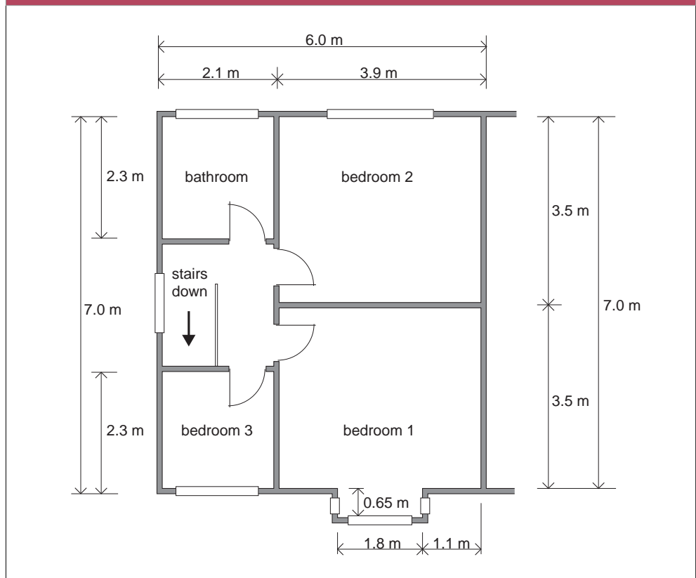
Diagram C3 Semi-detached house first floor plan
