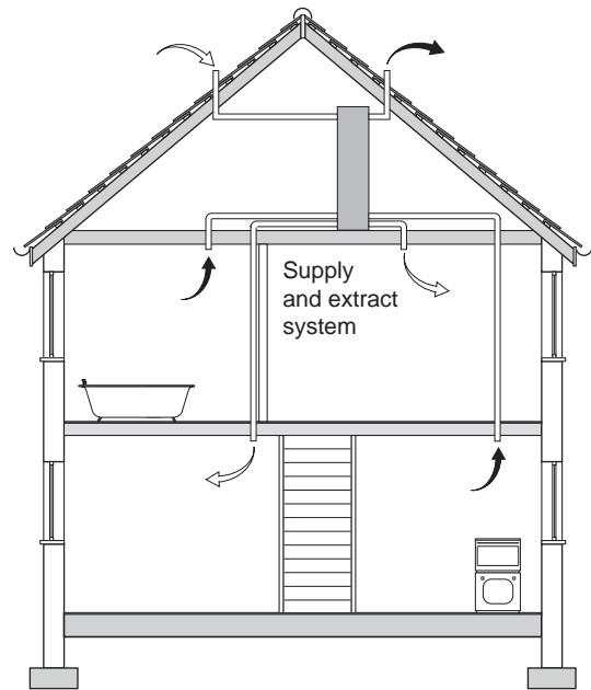
System 4 continuous mechanical supply and extract with heat recovery
