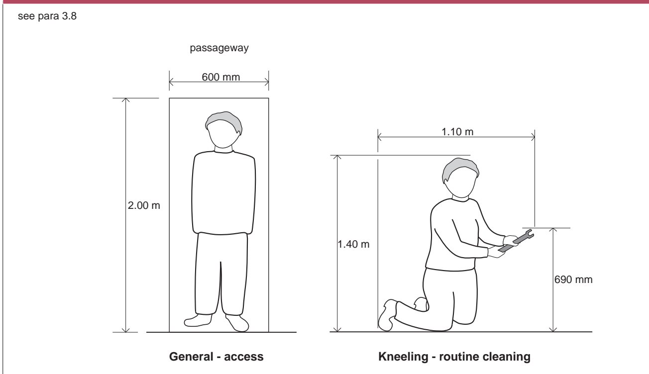
Diagram 3.1 Space for access (minimum dimensions)
